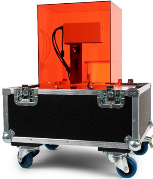
Image 17. Engraving Station
